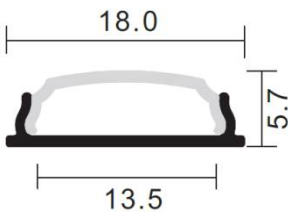
Dimension Drawing:
